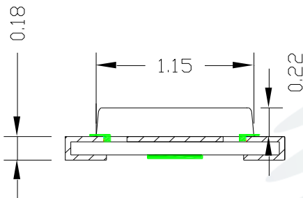
Fig.1-3 Side view 侧面视图
